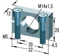
MB14 *€ 15,95 Klemflens
