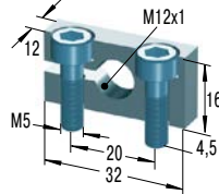
MB12 *€ 13,39 Klemflens
