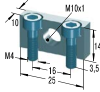
MB10SC2 *€ 12,78 Montageblok
