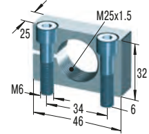
MB25 Clamp Mount
