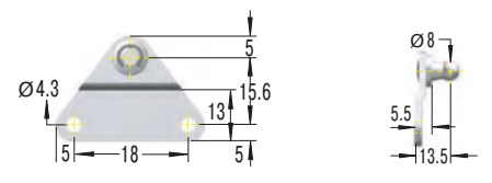
OG5-V4A Side Bracket with Ball
