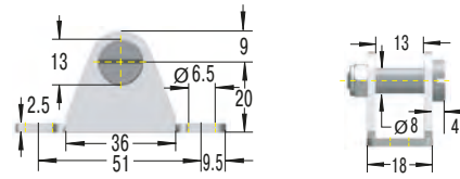
MA10 Bearing Shoe
