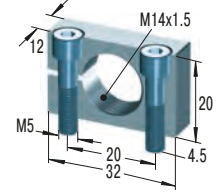
MB14 Clamp Mount
