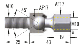
F10 Inline Ball Joint
