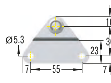
OG8-V4A Side Bracket with Ball
