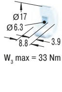
PP225 Nylon Button
