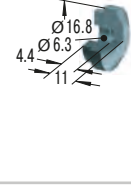
PS20 Steel Button
