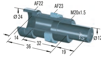
BV20SC Side Load Adaptor
