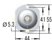
PG8-V4A Round Bracket with Ball
