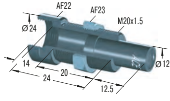
BV20 Side Load Adaptor
