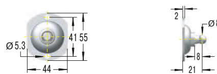
PG5-V4A Round Bracket with Ball
