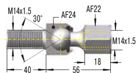
F14 Inline Ball Joint
