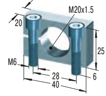
MB20 Clamp Mount
