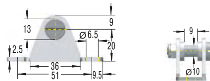
ME10 Bearing Shoe
