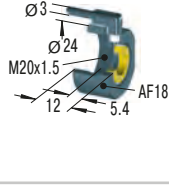
PP225 Nylon Button
