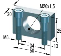
MB20SC2 *€ 17,62 Montageblock
