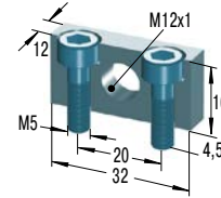
MB12SC2 *€ 14,23 Montageblock
