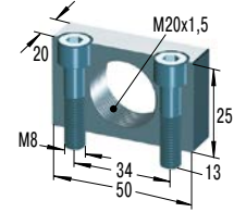
MB20SC2 *€ 17,62 Montageblock
