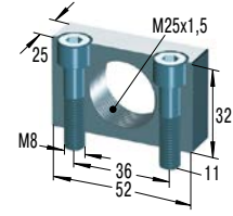
MB25SC2 *€ 25,04 Montageblock
