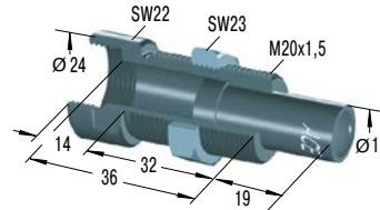
BV20SC *€ 52,59 Geleidingspen
