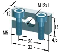
MB12 *€ 14,23 Klemflens
