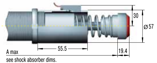
Switch Stop Collar
