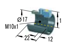
Switch Stop Collar inc. Proximity Switch
