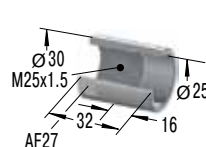
Stop Collar
