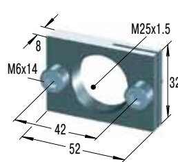
Rectangular Flange
