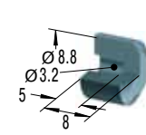
Steel Button
