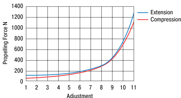
Propelling Force at 12.5 mm/s
