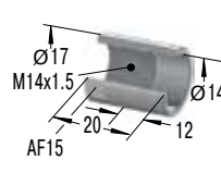
Stop Collar
