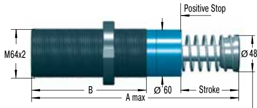
Standard Dimensions
