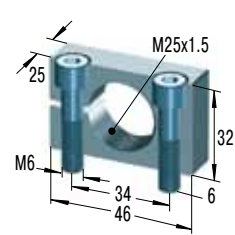
Clamp Mount
