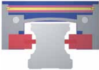
Example: Bosch Rexroth installation
