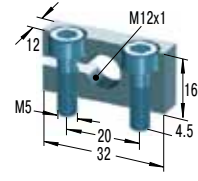
Clamp Mount
