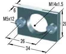
Rectangular Flange
