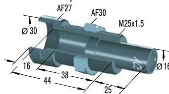
BV25SC Side Load Adaptor
