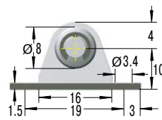
NA3,5 Angle Bracket with Ball
