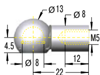
G5-VA Ball Socket
