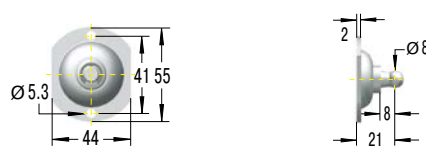
PG5 Round Bracket with Ball
