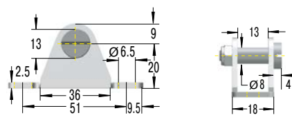
MA10-V4A Bearing Shoe
